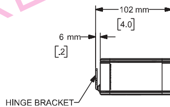
Left View
